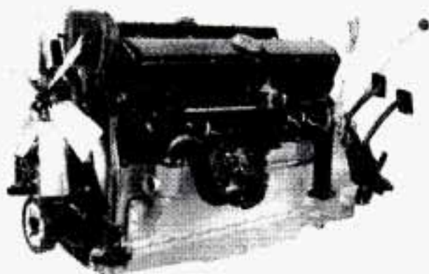
45° V-16 Engine
